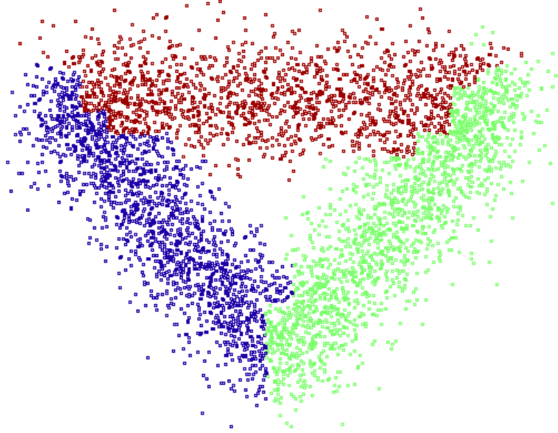
FIGURE 3.5: Waveform subset 1, relevant variables: labeling data using \text{GTM}_1
