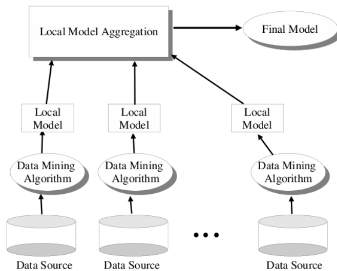
FIGURE 1.5: Distributed Data Mining Framerwork
